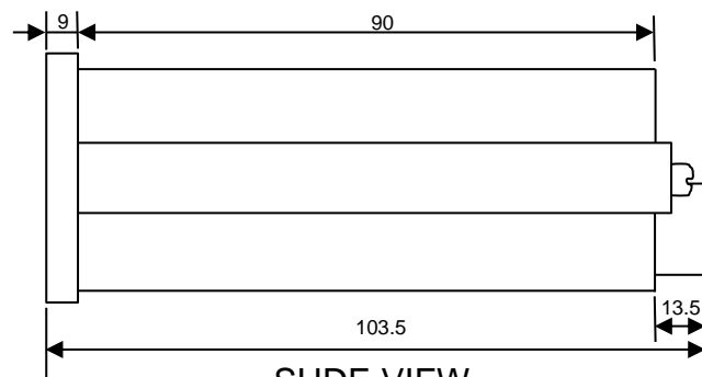
SUDE VIEW
